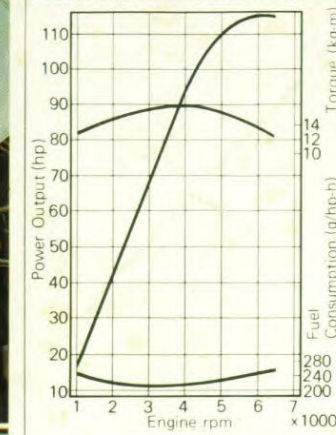
2000cc ENGINE PERFORMANCE CURVES
